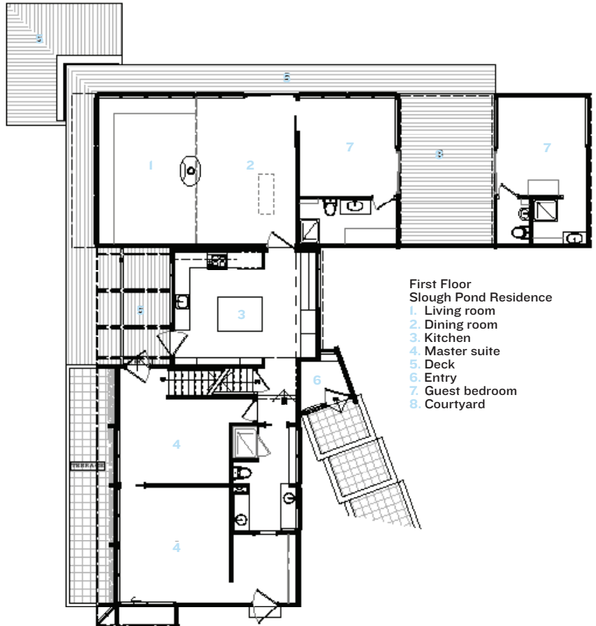
Above, the deep, cantilevered built-in sofa in the Hebbeln wing seats plenty of guests. Below, the plan shows the original house running across the top, with the new kitchen, entry, and master suite below.
